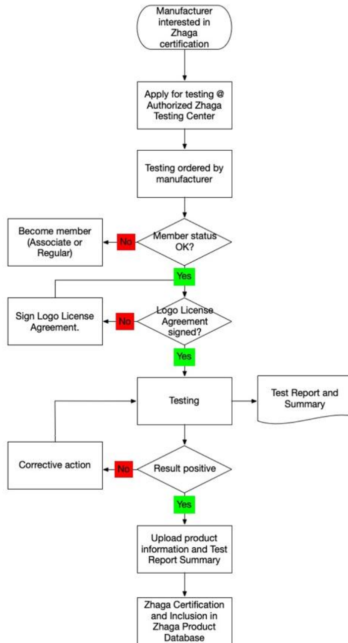
Figure 4-1: Process for Zhaga certification of a product.
