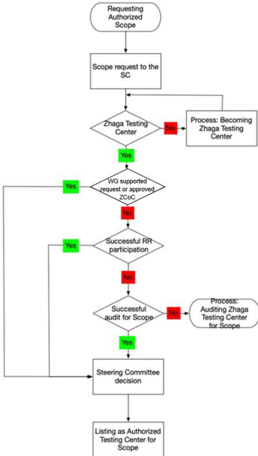
Figure 2-2: Process to request an Authorized Scope.
